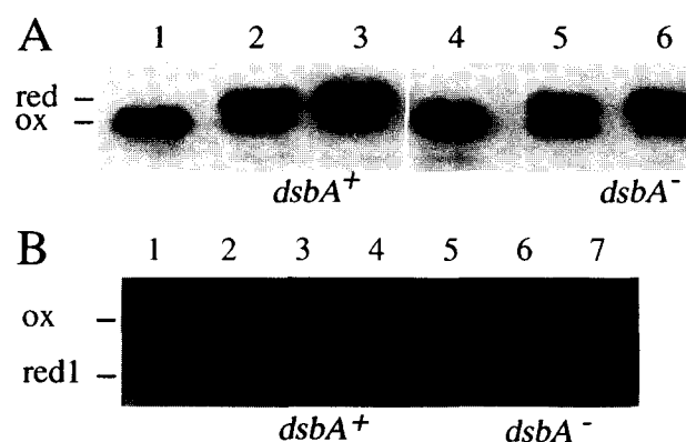
Fig. 2. Periplasmic fraction contains a factor(s) that reduces DsbA in vitro. Periplasmic fractions were prepared from CU141 (wild-type; lanes 2 and 3 of A and lanes 2–4 of B) or SS140 ( dsbA-::Tn5 ; lanes 5 and 6 of A and lanes 5–7 of B). Purified and oxidized DsbA (0.2 µg) was incubated, in a final volume of 50 µl of 3 mM Mops (pH 7), with 3 mM iodoacetic acid and the following amounts of periplasmic preparations: lanes 1 and 4 of A as well as lane 1 of B, none; lanes 2 and 5 of A, a culture-equivalent of 0.4 ml; lanes 3 and 6 of A, a culture-equivalent of 1.6 ml; lanes 2 and 5 of B, a culture-equivalent of 0.45 ml; lanes 3 and 6 of B, a culture equivalent of 1.35 ml. Redox states of DsbA were analyzed either by non-reducing SDS-PAGE (A) or native PAGE (B).
